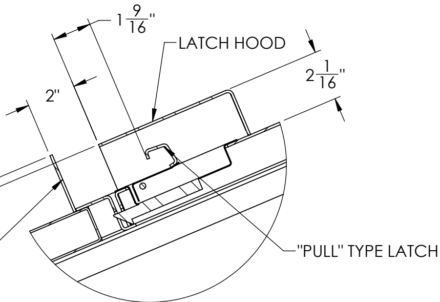
DETAIL B
